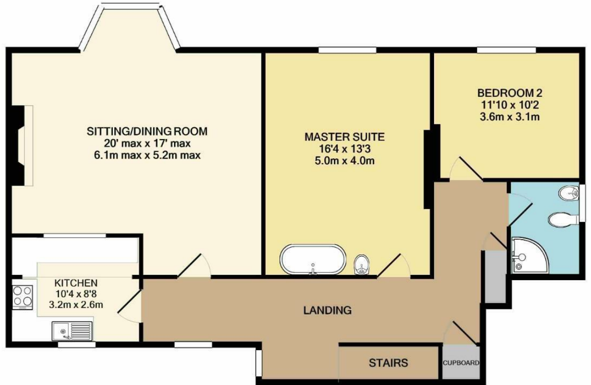
1ST FLOOR APPROX. FLOOR AREA 1081 SQ.FT. (100.5 SQ.M.)
